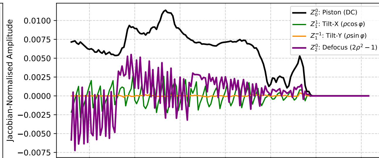
Zernike Packet Vector (Ray m = 45 )
